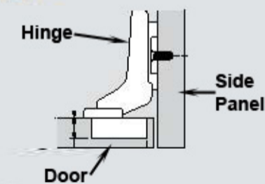
Inset Hinge
